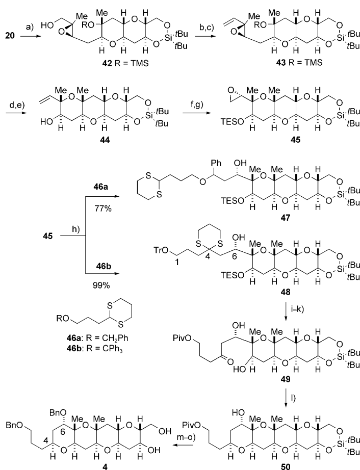
Scheme 7. Synthesis of the ABCD-ring fragment 4 : a) m CPBA, \text{NaHCO}_3 , \text{CH}_2\text{Cl}_2 , 0^\circ\text{C} , 96 % (d.r. 96:4); b) \text{SO}_3\cdot\text{py} , \text{Et}_3\text{N} , DMSO, 0^\circ\text{C} to RT; c) \text{Ph}_3\text{P}^+\text{CH}_3\cdot\text{Br}^- , KHMDS, THF, -80^\circ\text{C} to RT, 87 % (2 steps); d) n\text{Bu}_4\text{NF} , THF, -10^\circ\text{C} , 100 %; e) PPTS, \text{CH}_2\text{Cl}_2 , 74 %; f) t BuOOH, [\text{VO}(\text{acac})_2] , \text{CH}_2\text{Cl}_2 , 35^\circ\text{C} , 85 % (d.r. 93:7); g) TESCl, \text{Et}_3\text{N} , DMAP, \text{CH}_2\text{Cl}_2 , 96 %; h) 46b , n\text{BuLi} , THF, 0^\circ\text{C} , 48 (99 %); i) p TsOH· \text{H}_2\text{O} , MeOH, \text{CH}_2\text{Cl}_2 , RT, 97 %; j) PivCl, DMAP, py, \text{CH}_2\text{Cl}_2 , 0^\circ\text{C} , 98 %; k) \text{Hg}(\text{ClO}_4)_2 , THF, \text{H}_2\text{O} , 0^\circ\text{C} , 90 %; l) \text{Et}_3\text{SiH} , \text{SnCl}_4 , \text{CH}_2\text{Cl}_2 , -40^\circ\text{C} , 91 %; m) DIBALH, \text{CH}_2\text{Cl}_2 , -80^\circ\text{C} , 98 %; n) NaH, BnBr, DMF, 86 %; o) n\text{Bu}_4\text{NF} , THF, RT, 97 %. KHMDS = potassium hexamethyldisilazide, m CPBA = meta -chloroperoxybenzoic acid, PivCl = pivaloyl chloride, PPTS = pyridinium p toluenesulfonate, TESCl = chlorotriethylsilane.
