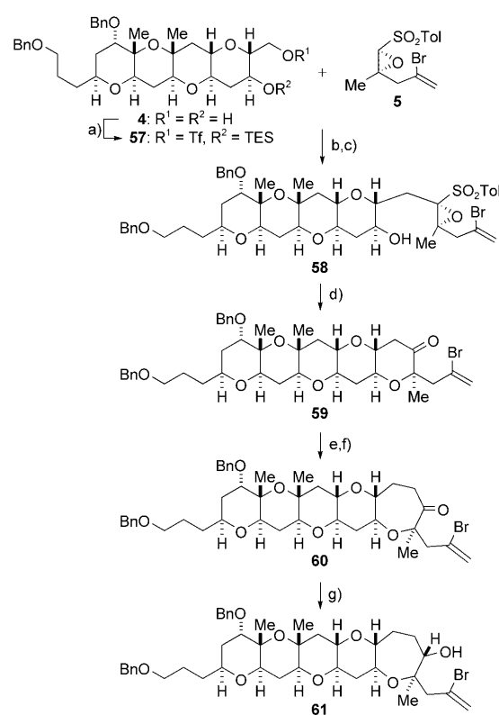
Scheme 9. Synthesis of the ABCDE-ring system 61 : a) \text{Tf}_2\text{O} , 2,6-lutidine, -80^{\circ}\text{C} , \text{CH}_2\text{Cl}_2 , then \text{TESOTf} , 92%; b) 5 , n BuLi, THF, HMPA, -100^{\circ}\text{C} , 91%; c) p TsOH- \text{H}_2\text{O} , \text{CH}_2\text{Cl}_2 , MeOH, RT, 91%; d) \text{BF}_3\cdot\text{OEt}_2 , \text{CH}_2\text{Cl}_2 , -80^{\circ}\text{C} , 98%; e) \text{TMSCHN}_2 , \text{BF}_3\cdot\text{OEt}_2 , \text{CH}_2\text{Cl}_2 , -20^{\circ}\text{C} , 53%; f) n Bu 4 NF, THF, AcOH, RT, 97%; g) \text{NaBH}_4 , \text{CH}_2\text{Cl}_2 , MeOH, -80^{\circ}\text{C} , 59% (+ isomer 41%). \text{TMSCHN}_2 =trimethylsilyldiazomethane.
