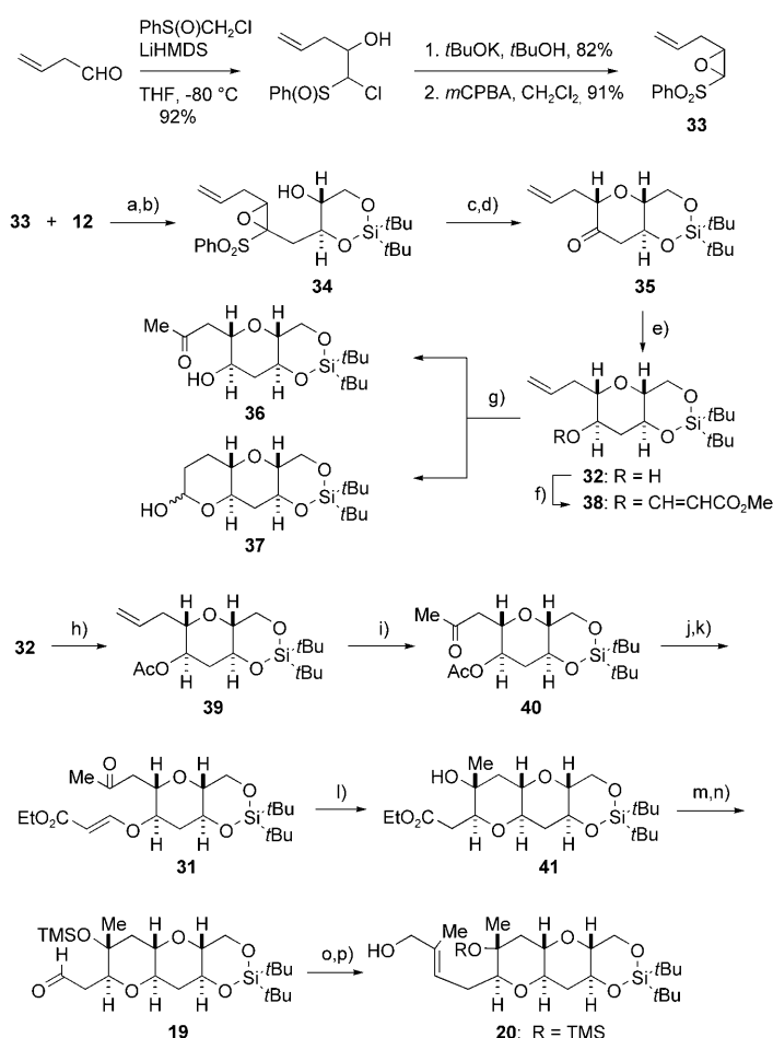
Scheme 6. Synthesis of the CD rings—the third approach: a) n BuLi, THF, HMPA, -100^{\circ}\text{C} , 94%; b) p TsOH \cdot H 2 O, CH 2 Cl 2 , MeOH, RT, 94%; c) MgBr 2 \cdot OEt 2 , LiBr, CH 2 Cl 2 , -15 to 0^{\circ}\text{C} , 94%; d) DBU, CH 2 Cl 2 , 0^{\circ}\text{C} , 100% (d.r. 94:6); e) NaBH 4 , MeOH, CH 2 Cl 2 , -80^{\circ}\text{C} , 91%; f) methyl propiolate, NMM, CH 2 Cl 2 , RT, 90%; g) PdCl 2 , CuCl, CH 3 CN, H 2 O, RT, 36 (44%), 37 (44%); h) Ac 2 O, py, DMAP, CH 2 Cl 2 , 86%; i) PdCl 2 , DMF, H 2 O, RT, 73%; j) K 2 CO 3 , MeOH, RT, 93%; k) ethyl propiolate, NMM, CH 2 Cl 2 , RT, 97%; l) SmI 2 , THF, MeOH, 0^{\circ}\text{C} , 100%; m) TMSOTf, 2,6-lutidine, 0^{\circ}\text{C} , CH 2 Cl 2 , 96%; n) DIBALH, CH 2 Cl 2 , -80^{\circ}\text{C} , 99%; o) 9 , toluene, RT, 96%; p) DIBALH, CH 2 Cl 2 , -80^{\circ}\text{C} , 93%. DMAP = 4-dimethylaminopyridine; NMM = N -methylmorpholine.
