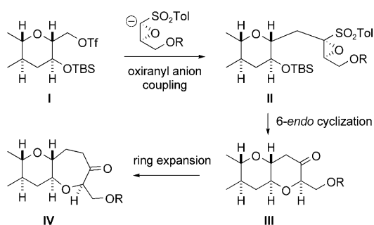
Scheme 1. Synthesis of six- and seven-membered rings by an oxiranyl anion strategy.
