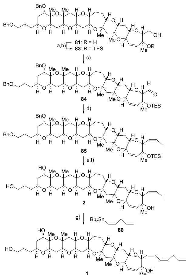
Scheme 13. Completion of the total synthesis: a) TESOTf, 2,6-lutidine, \text{CH}_2\text{Cl}_2 , 0^\circ\text{C} , 95%; b) PPTS, \text{CH}_2\text{Cl}_2 , MeOH, 0^\circ\text{C} , 98%; c) TPAP, NMO, \text{CH}_2\text{Cl}_2 , RT, 93%; d) \text{Ph}_3\text{P}^+\text{CH}_2\text{I}^- , NaHMDS, THF, -80^\circ\text{C} to RT, 68%; e) DDQ, \text{H}_2\text{O} , diallyl ether, DCE, 50^\circ\text{C} ; f) p\text{TsOH}\cdot\text{H}_2\text{O} , \text{CH}_2\text{Cl}_2 , MeOH, RT, 78% (2 steps); g) 86 , [\text{Pd}_2(\text{dba})_3]\cdot\text{CHCl}_3 , \text{P}(\text{furyl})_3 , CuI, DMSO, 40^\circ\text{C} , 68%. dba = dibenzylideneacetone, DCE = 1,2-dichloroethane. TPAP = tetra- n -propylammonium perruthenate, NMO = 4-methylmorpholine- N -oxide.
