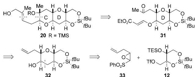
Scheme 5. The third approach for the CD-ring fragment 20 .
