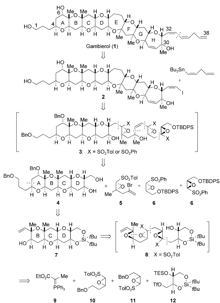
Scheme 2. Retrosynthetic analysis of gambierol ( 1 ).
