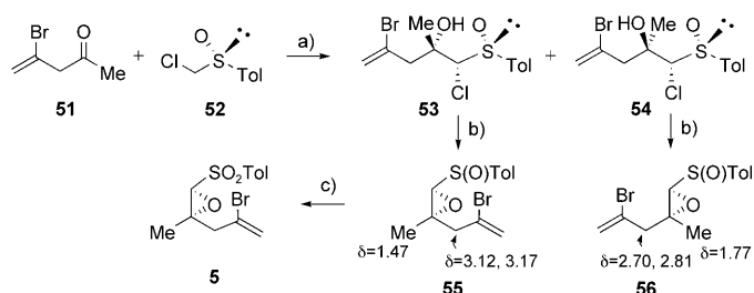
Scheme 8. Preparation of epoxy sulfone 5 : a) 52 , LiHMDS, THF, -80^{\circ}\text{C} , then 51 , 53 (40%), 54 (40%); b) t BuOK, t BuOH, \text{CH}_2\text{Cl}_2 , 0^{\circ}\text{C} , 55 (90%), 56 (83%); c) m CPBA, \text{CH}_2\text{Cl}_2 , 0^{\circ}\text{C} , 94%. LDA=lithium diisopropylamide.
