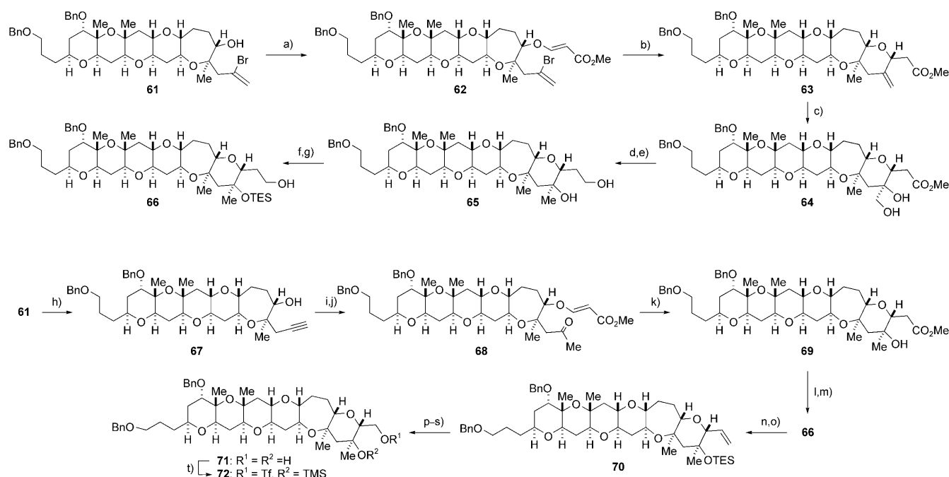
Scheme 10. Synthesis of the ABCDEF-ring triflate 72 : a) methyl propiolate, NMM, CH 2 Cl 2 , RT, 95%; b) n Bu 3 SnH, AIBN, toluene, 110°C, 81%; c) OsO 4 , NMO, THF, H 2 O, RT, 88%; d) MsCl, Et 3 N, CH 2 Cl 2 , -10°C, 96%; e) LiEt 3 BH, THF, 0°C, 98%; f) TESOTf, 2,6-lutidine, CH 2 Cl 2 , 0°C, 94%; g) PPTS, MeOH, CH 2 Cl 2 , 0°C, 95%; h) n Bu 4 NF·3H 2 O, DMF, 60°C, 99%; i) Hg(OTf) 2 , TMU, CH 2 Cl 2 , MeCN, H 2 O, RT, 82%; j) methyl propiolate, NMM, CH 2 Cl 2 , RT, 82%; k) SmI 2 , THF, MeOH, 0°C, 100%; l) TESOTf, 2,6-lutidine, CH 2 Cl 2 , 0°C, 92%; m) DIBALH, CH 2 Cl 2 , 0°C, 96%; n) o -NO 2 PhSeCN, n Bu 3 P, CH 2 Cl 2 , py, RT; o) H 2 O 2 , NaHCO 3 , THF, RT, 85% (2 steps); p) OsO 4 , NMO, THF, H 2 O, RT; q) NaIO 4 , MeOH, H 2 O, RT; r) NaBH 4 , CH 2 Cl 2 , MeOH, RT, 98% (3 steps); s) p TsOH-H 2 O, CH 2 Cl 2 , MeOH, RT, 100%; t) Tf 2 O, 2,6-lutidine, CH 2 Cl 2 , -80°C, then TMSOTf, 95%. AIBN = 2,2'-azobisisobutyronitrile, TMU = 1,1,3,3,3-tetramethylurea.
